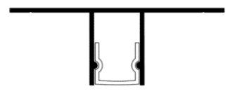
LED FLUSH SCREED
