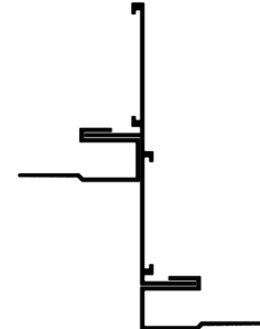
DRYWALL CEILING TRANSITION TO DRYWALL
