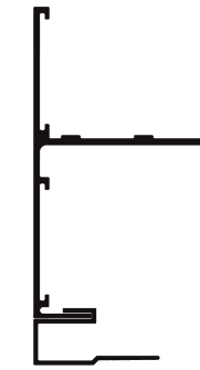
UNIVERSAL LIGHT COVE DRYWALL EDGE
