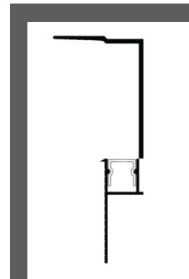
LED CEILING MOLD
