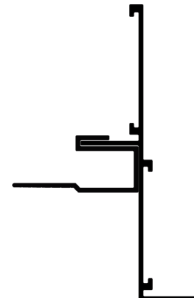
ACOUSTICAL CEILING TRANSITION TO DRYWALL
