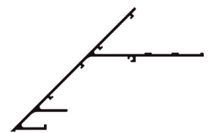
UNIVERSAL LIGHT COVE DRYWALL KNIFE EDGE
