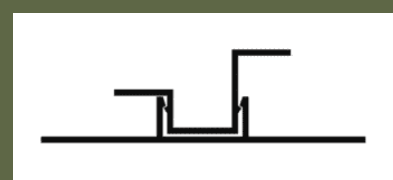
OFFSET PANEL SCREED
