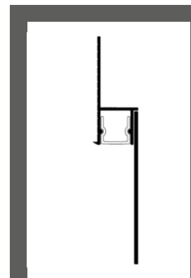
LED BASE MOLD
